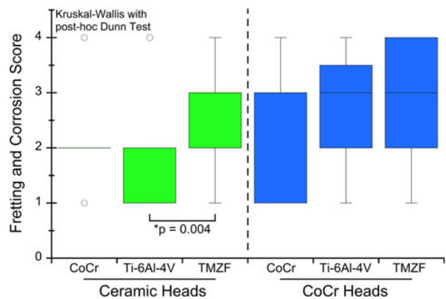
Fig. 4 A boxplot illustrating femoral stem taper fretting and corrosion score versus stem alloy for the ceramic and metal head cohorts is presented.
